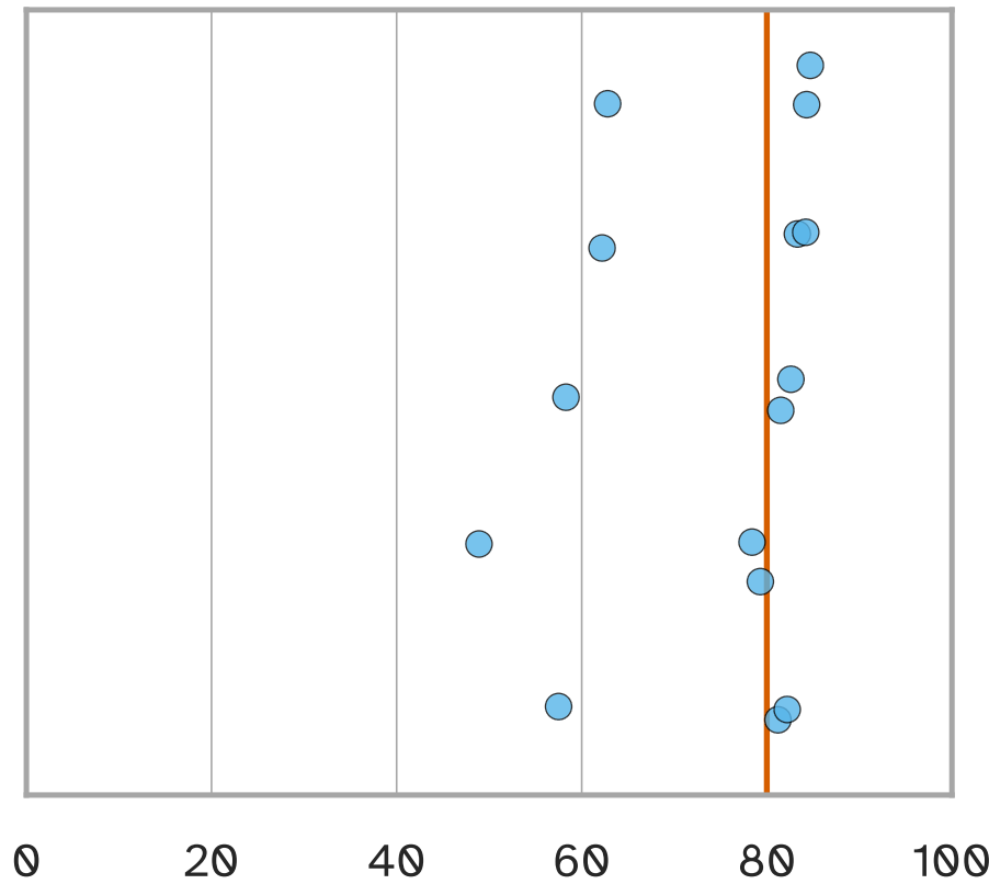
Normal
